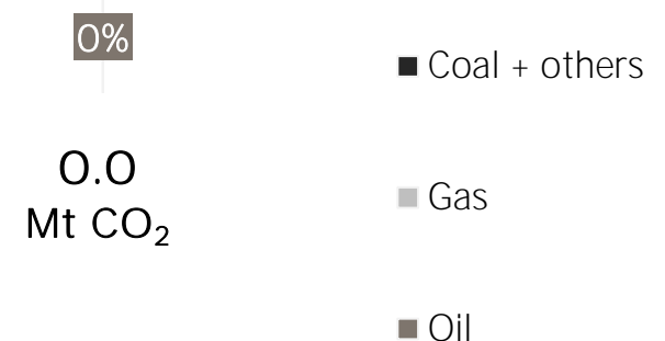
Elec. & heat generation CO 2 emissions in 2017
