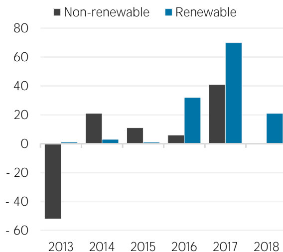
Net capacity change (MW)
