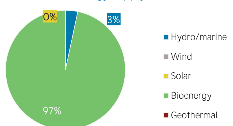
Renewable energy supply in 2019
