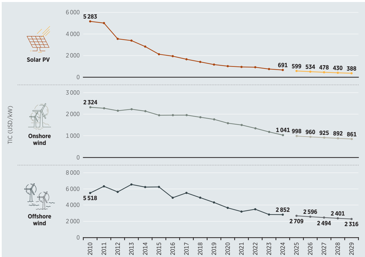
Figure 1.19 Historical and projected global TIC values
