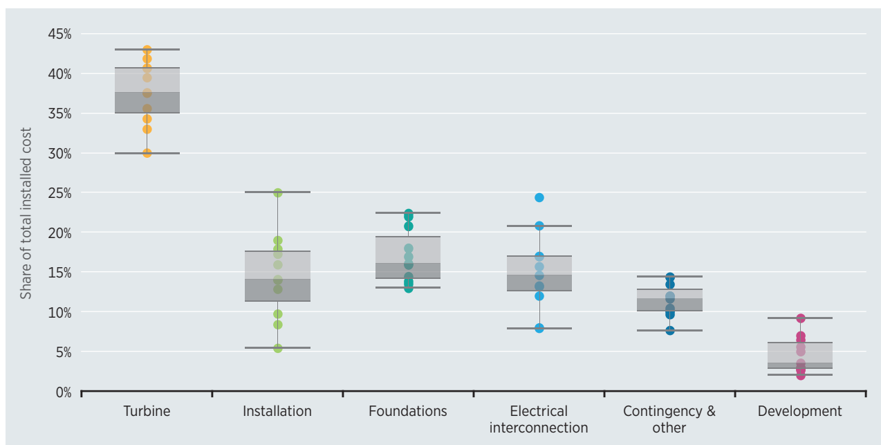
Figure 4.6 Comparative breakdown of offshore wind total installed cost from selected market studies
