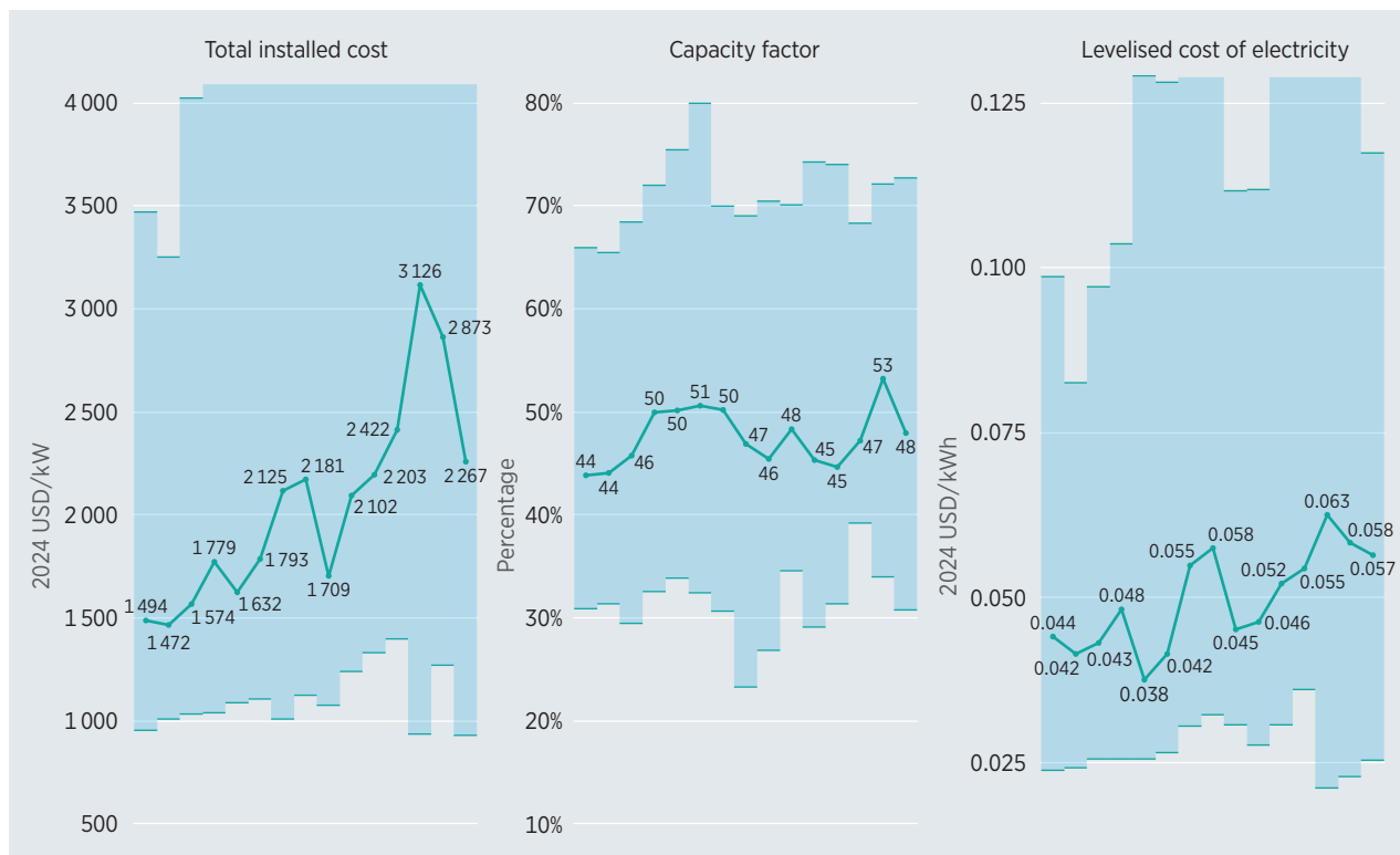
Figure 6.1 Global weighted average and range of total installed costs, capacity factors and LCOEs for hydropower, 2010–2024
