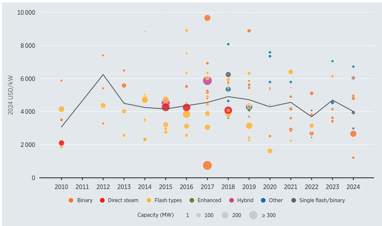
Figure 7.2 Geothermal power, total installed costs by project, technology and capacity, 2010–2024
