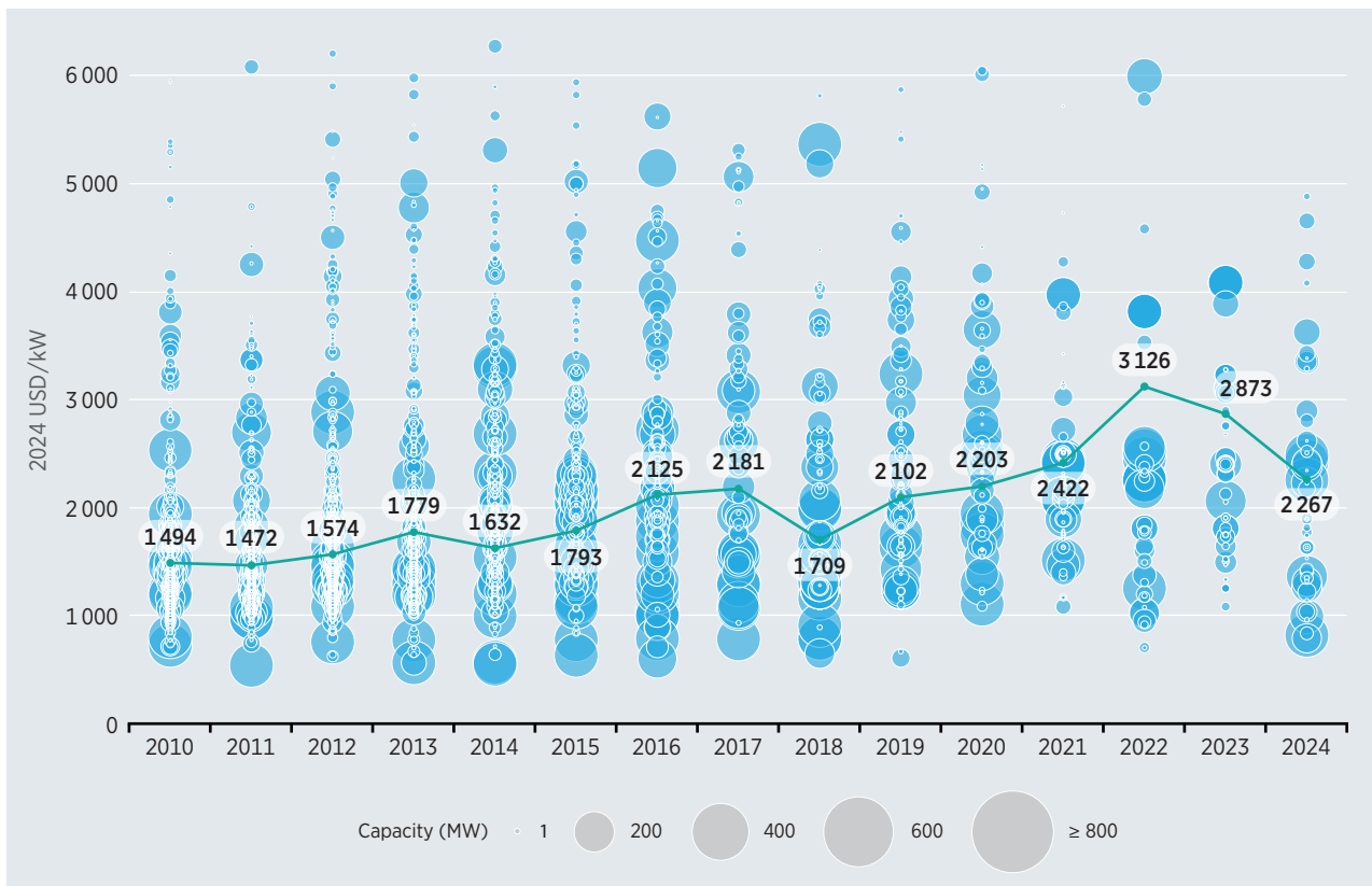
Figure 6.2 Total installed costs by project and global weighted average for hydropower, 2010–2024
