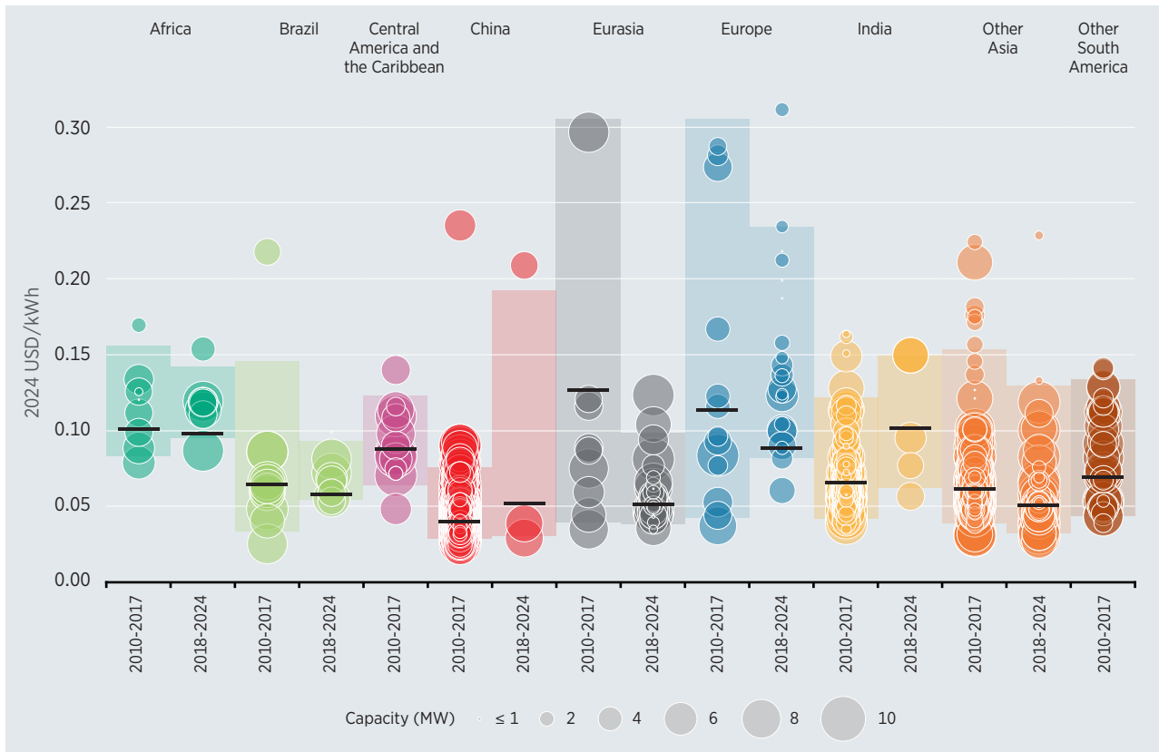
Figure 6.9 Small hydropower project LCOE and weighted averages by country/region, 2010-2024
