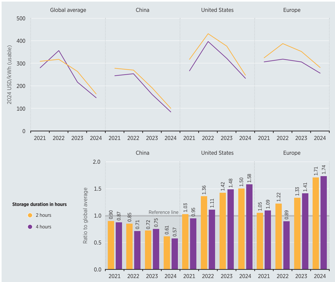
Figure 9.3 Turnkey battery storage system prices by market and duration, 2021–2024
