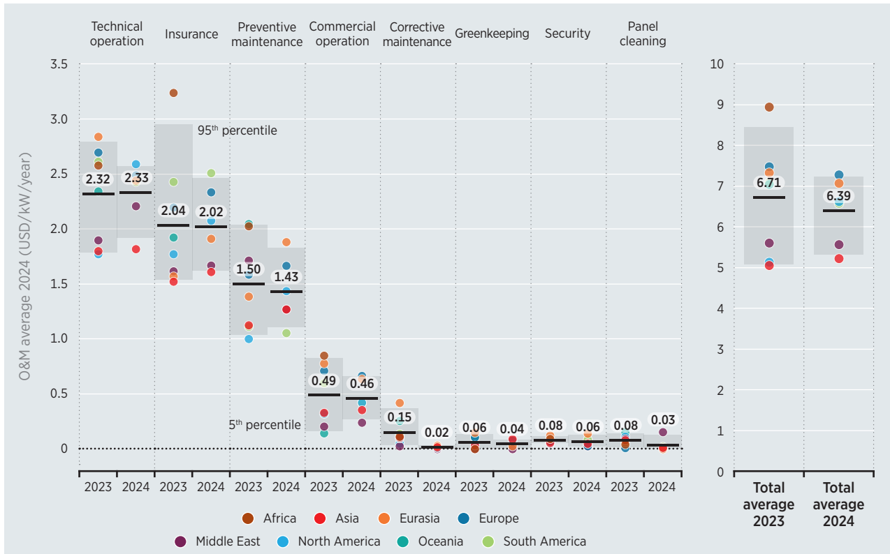
Figure 3.7 Survey results for the average, all-in O&M costs for utility-scale solar PV by cost category and region, 2023-2024
