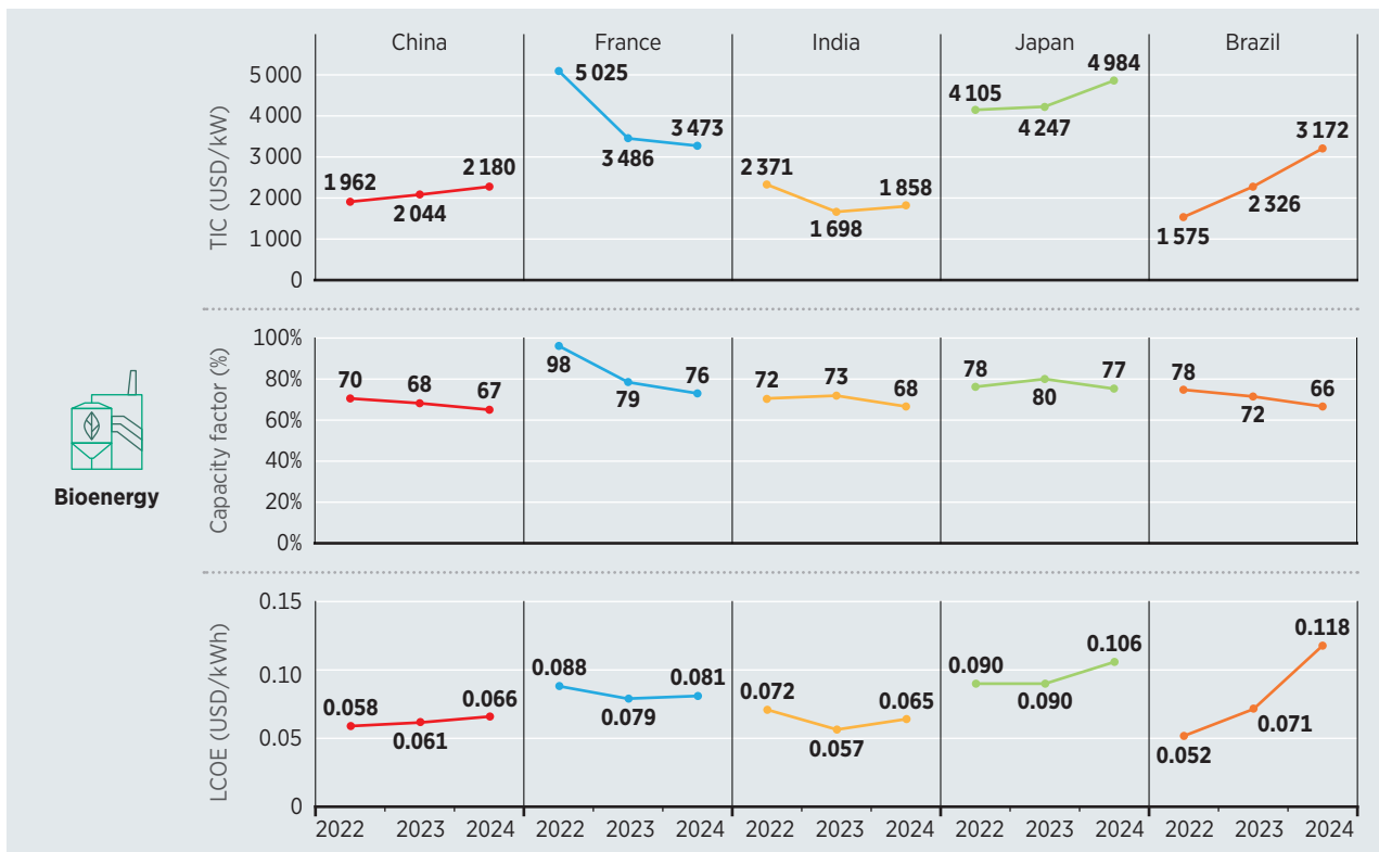
Figure 1.18 Bioenergy cost and performance trajectories in selected countries, 2022-2024
