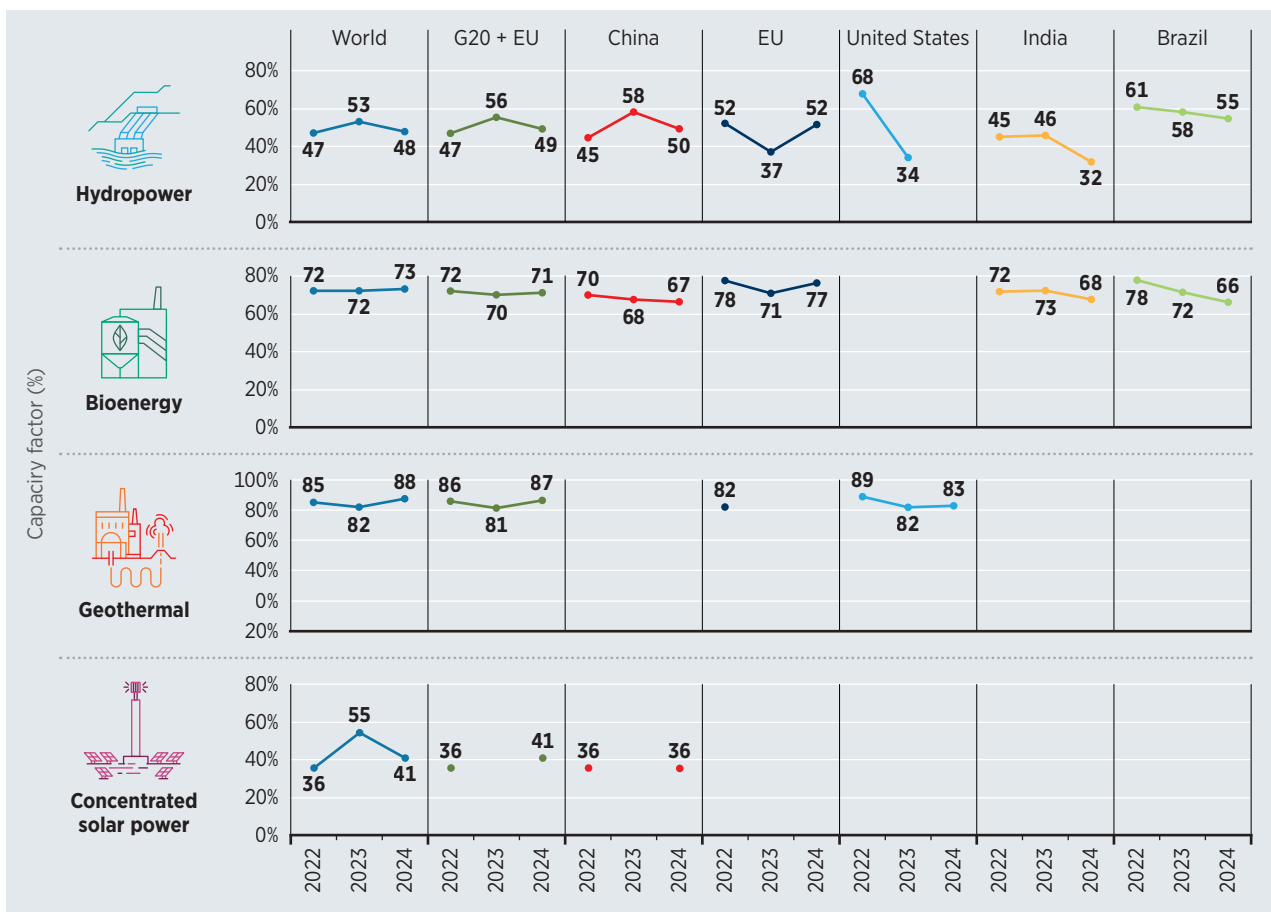
Figure 1.5 Capacity factor trajectories of dispatchable technologies in selected regions, 2022-2024
