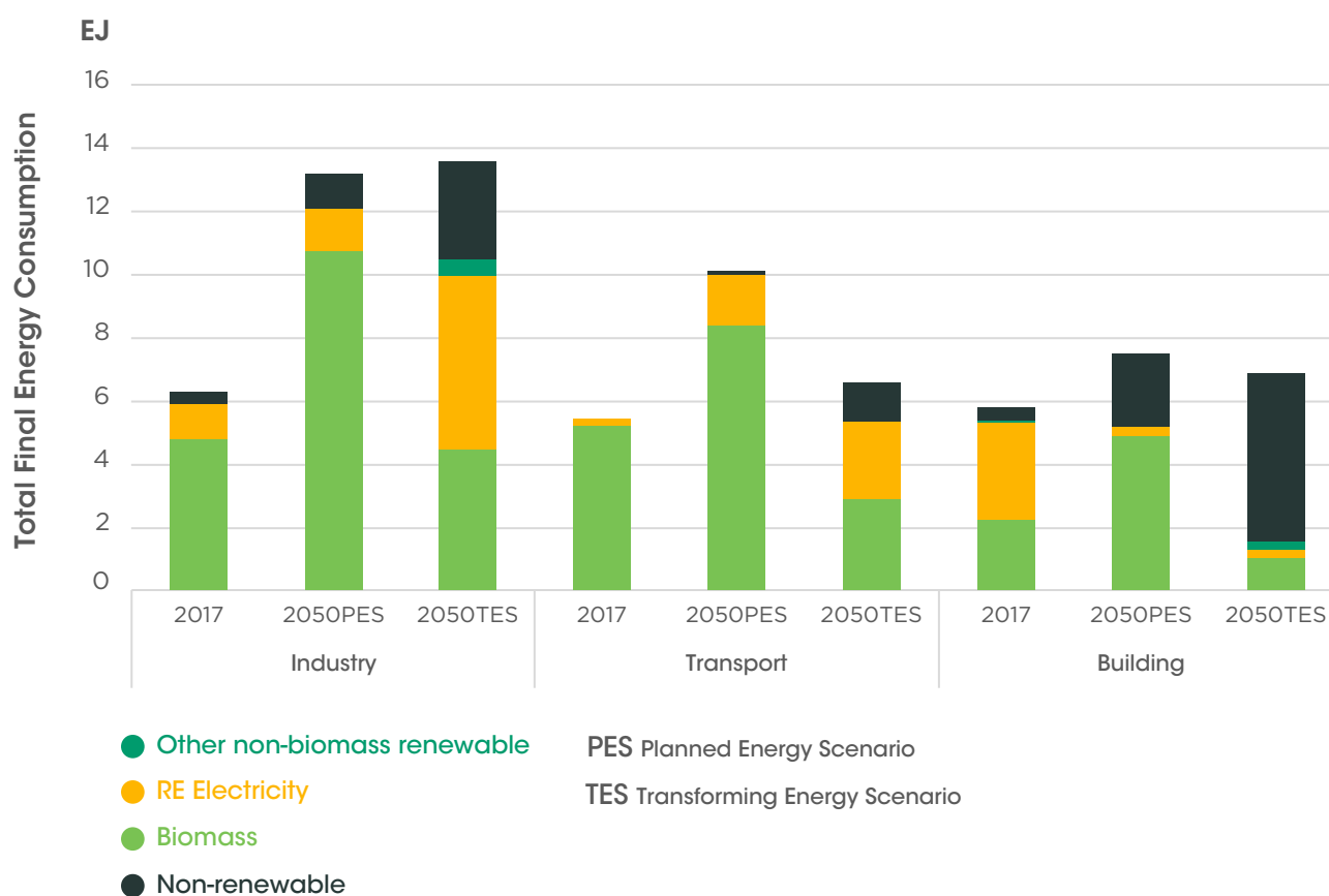
FIGURE 2: Energy Transformation Scenarios in Southeast Asia (TFEC)
