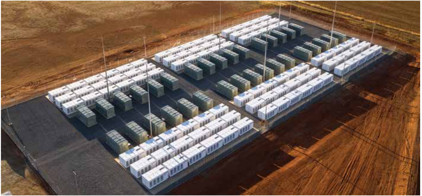
Figure 32: Hornsdale power reserve project in South Australia
