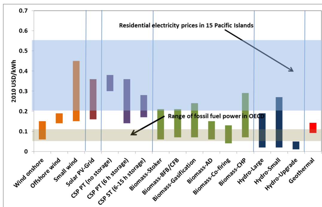
Figure 1: The typical levelised cost of renewable power generation technologies
