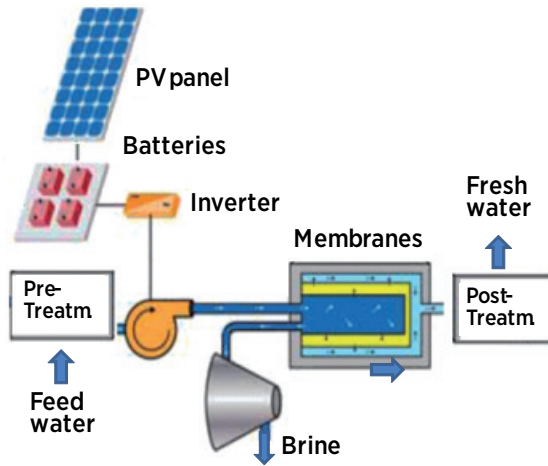
Figure 4 – Coupled PV and RO desalination plants (Al-Karaghoulis et al., 2011)
